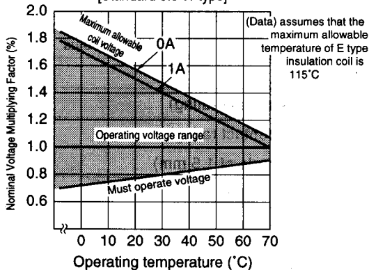
Range of operation temperature and voltage [Standard 0.5 W type]
