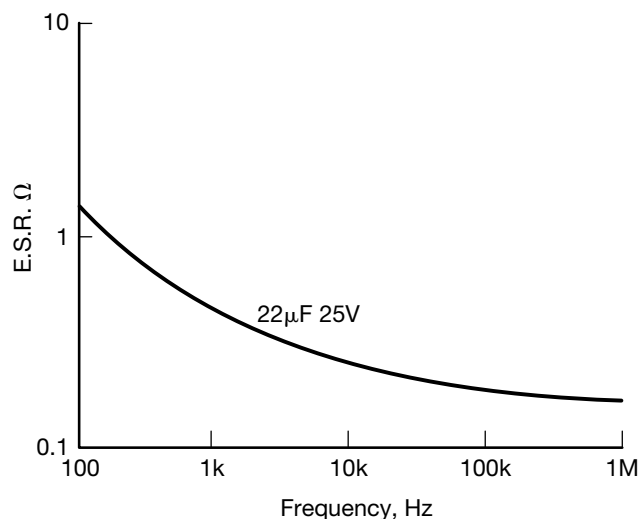
Figure 1. Typical relationship between ESR and frequency.
